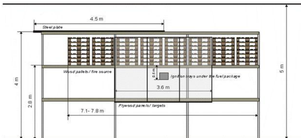
FIGURE F.T5.303.1 - SIDE VIEW OF THE CARGO FUEL PACKAGE IN A SIMULATED TRUCK
