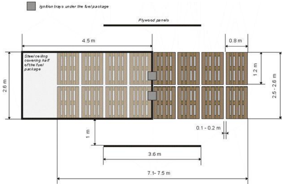
FIGURE F.T5.303.3 - TOP VIEW OF THE CARGO FUEL PACKAGE IN A SIMULATED TRUCK
