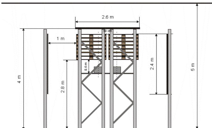
FIGURE F.T5.303.2 - END VIEW OF THE CARGO FUEL PACKAGE IN A SIMULATED TRUCK
