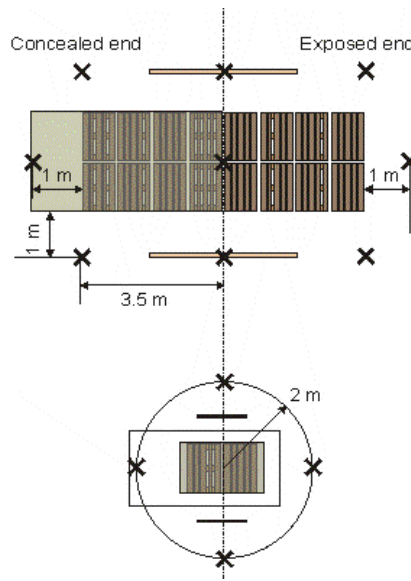
FIGURE F.T5.305.2 - THERMOCOUPLE LOCATIONS AT THE PLYWOOD TARGETS FOR DETERMINING IGNITION OF TARGETS
