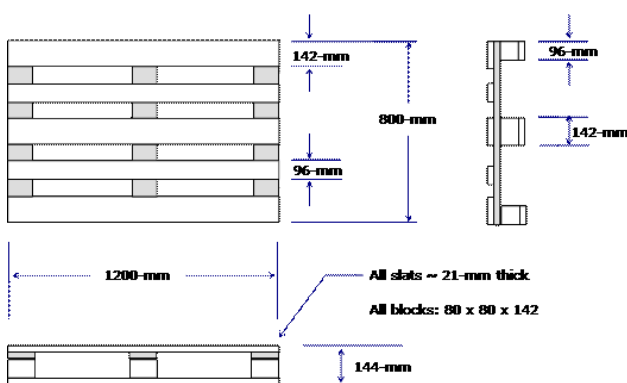
FIGURE F.T5. 3026.1 – TYPICAL DIMENSION OF STANDARD EUR PALLET
