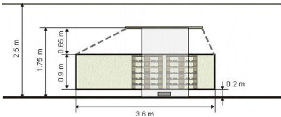
F.T5.303.4 - SIDE VIEW OF THE PASSENGER VEHICLE FUEL PACKAGE
