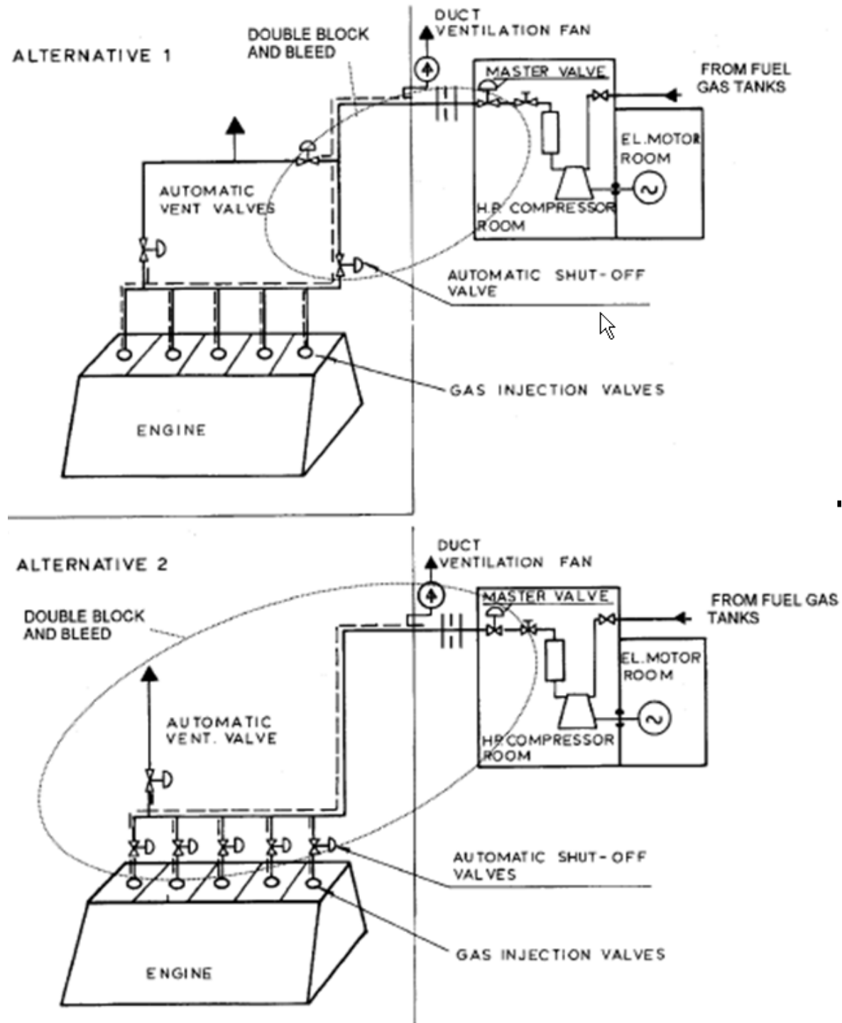
FIGURE F.F1.603.1 - ALTERNATIVE SUPPLY VALVE ARRANGEMENTS FOR HIGH-PRESSURE INSTALLATIONS (SINGLE ENGINE OR SEPARATE MASTER VALVE ARRANGEMENT)
