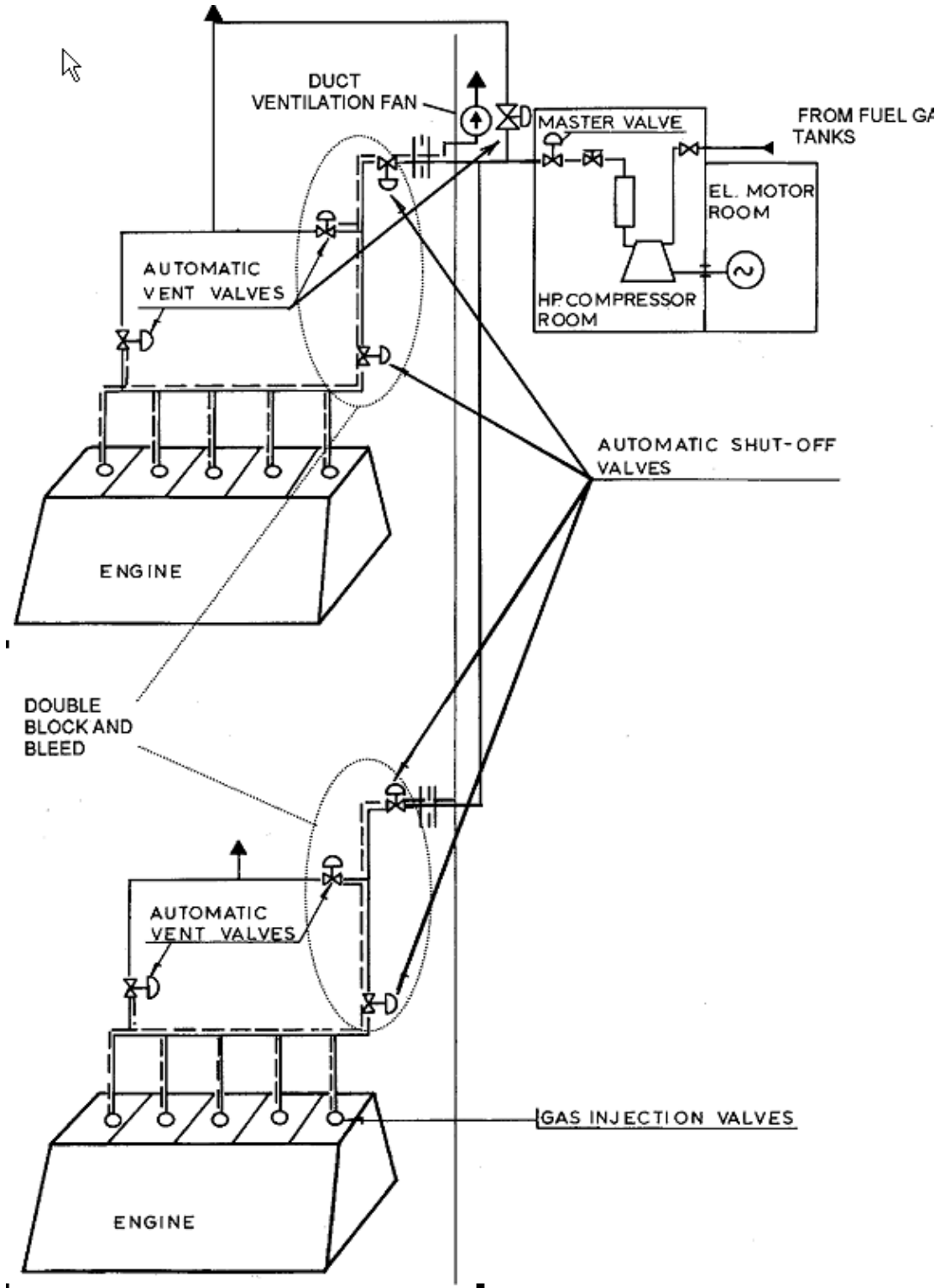
FIGURE F.F1.603.1 - ALTERNATIVE SUPPLY VALVE ARRANGEMENTS FOR HIGH-PRESSURE INSTALLATIONS (MULTI-ENGINE INSTALLATION)
